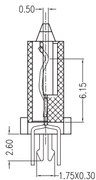
SECT C-C
